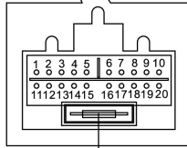
Power Fuse(15A)
